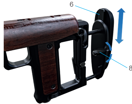
Pic. 22 Recoil pad height adjustment .
