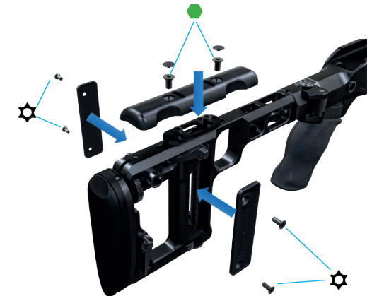
Pic. 40 The cheekpiece and buttstock panels are changed.
