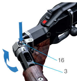
Pic.17 Unfold the buttstock.
