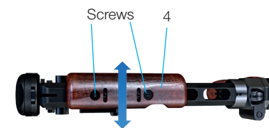
Pic. 20 Cheekpiece after adjustment (SIDEWAYS).
