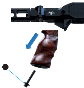
Pic. 37 The grip is removed.
